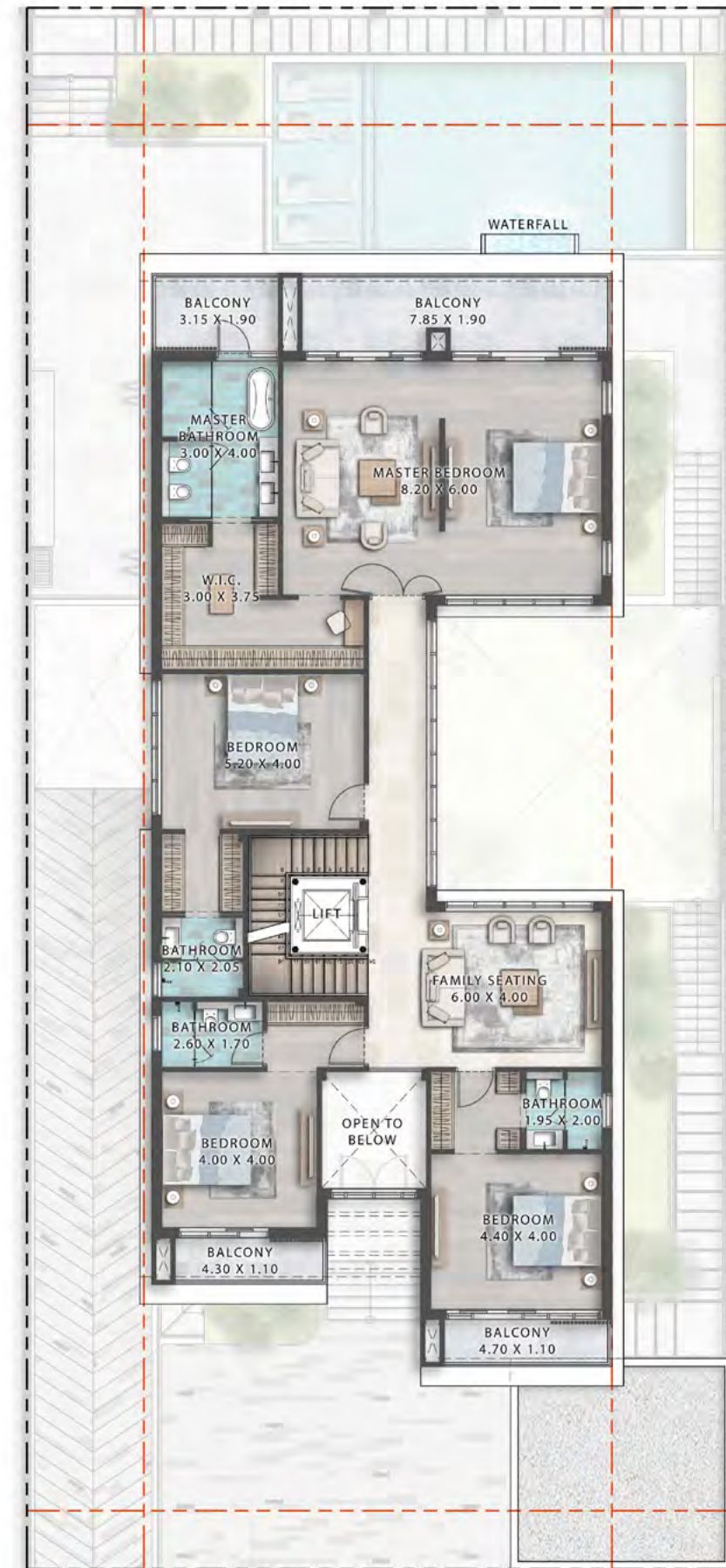
FIRST FLOOR
